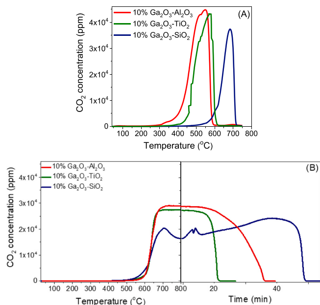
Fig. 15. Responses of CO 2 produced during temperature programmed oxidation with 3 %O 2 (in He) occurred after the TOS stability tests presented in Figs. 8–10 conducted at (A) 600 °C over 10 % Ga 2 O 3 -Al 2 O 3 catalyst and 660 °C over 10 % Ga 2 O 3 -SiO 2 and 10 % Ga 2 O 3 -TiO 2 catalysts and (B) 710 °C over 10 % Ga 2 O 3 -Al 2 O 3 , 10 % Ga 2 O 3 -SiO 2 and 10 % Ga 2 O 3 -TiO 2 catalysts. In (B), CO 2 responses above 800 °C were recorded as a function of time since catalysts needed to remain at 800 °C for 20–50 min until complete oxidation of carbon.
