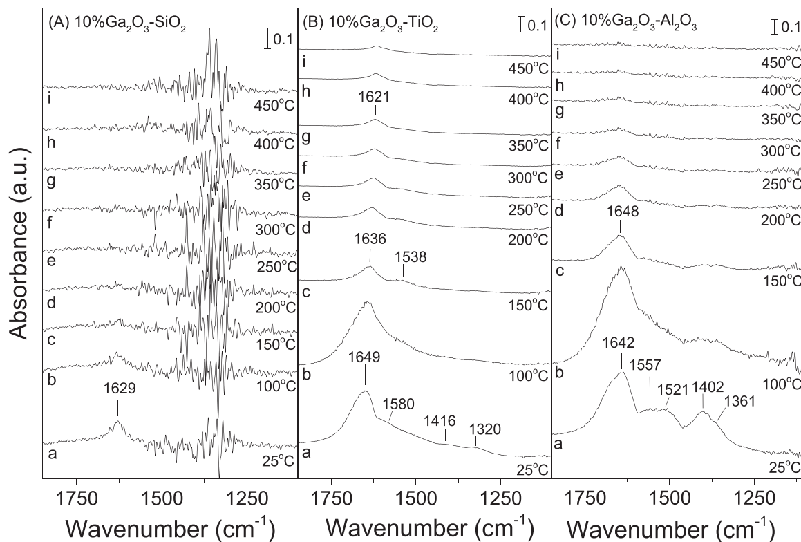
Fig. 3. DRIFT spectra obtained from (A) 10%Ga 2 O 3 -SiO 2 , (B) 10%Ga 2 O 3 -TiO 2 and (C) 10%Ga 2 O 3 -Al 2 O 3 catalysts following adsorption of CO 2 at 25 °C for 30 min and subsequent stepwise heating at the indicated temperatures under He flow.
