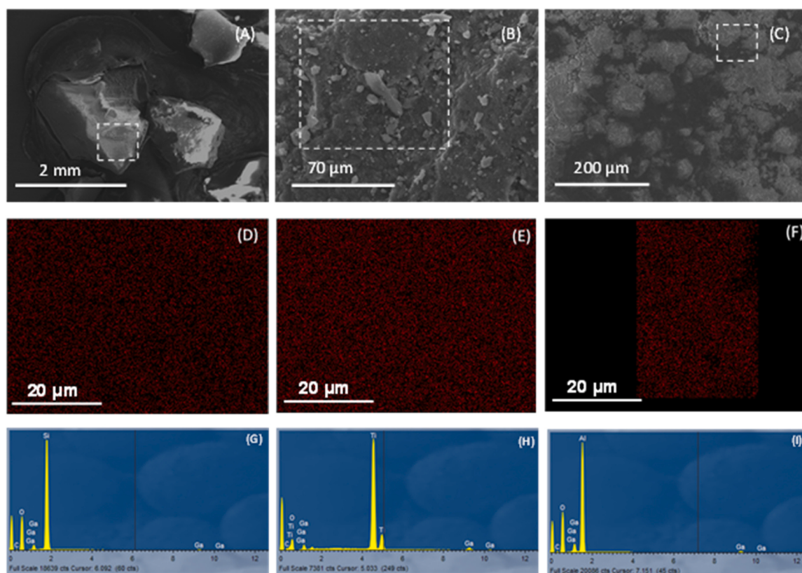
Fig. 13. SEM images with element mapping of Ga and EDS profiles obtained from the “fresh” (A, D, G) 10 % \text{Ga}_2\text{O}_3\text{-SiO}_2 (B, E, H) 10 % \text{Ga}_2\text{O}_3\text{-TiO}_2 and (C, F, I) 10 % \text{Ga}_2\text{O}_3\text{-Al}_2\text{O}_3 catalysts.
