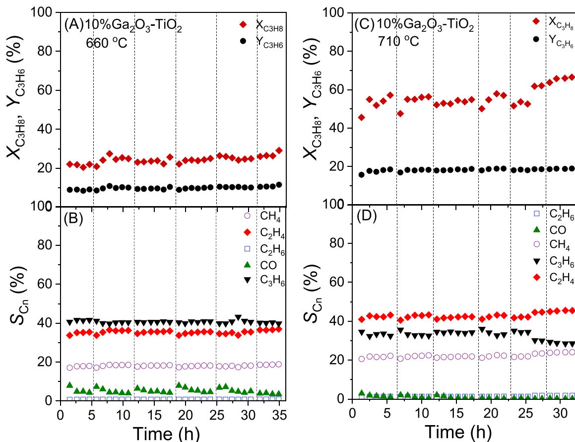
Fig. 10. TOS stability test of the 10%Ga 2 O 3 -TiO 2 catalyst conducted at (A, B) 660 °C and (C, D) 710 °C under conditions of oxidative dehydrogenation of C 3 H 8 with CO 2 . Alterations of (A, C) X_{\text{C}_3\text{H}_8} and Y_{\text{C}_3\text{H}_6} , and (B, D) products selectivity with time-on-stream. Experimental conditions: Same as in Fig. 5. Dashed vertical black lines indicate shutting down of the system overnight where the catalyst remained under He flow. (A) and (B) are reproduced from Ref [1].
